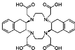
trans-anti-trans
