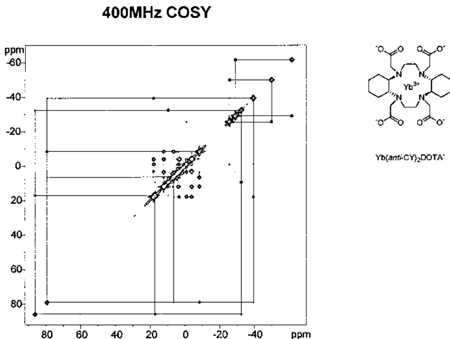
Fig. 7. COSY-NMR spectrum of Yb( trans-anti-trans CY) 2 DOTA - .
